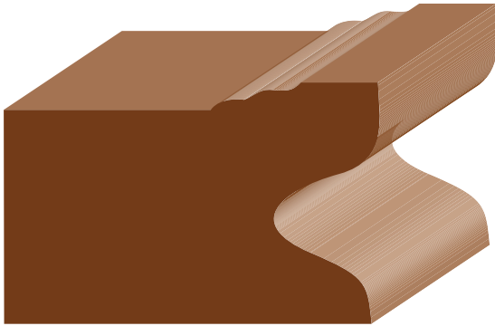
Brick Mould w/Key P-381PRKey 1-1/4 x 2
